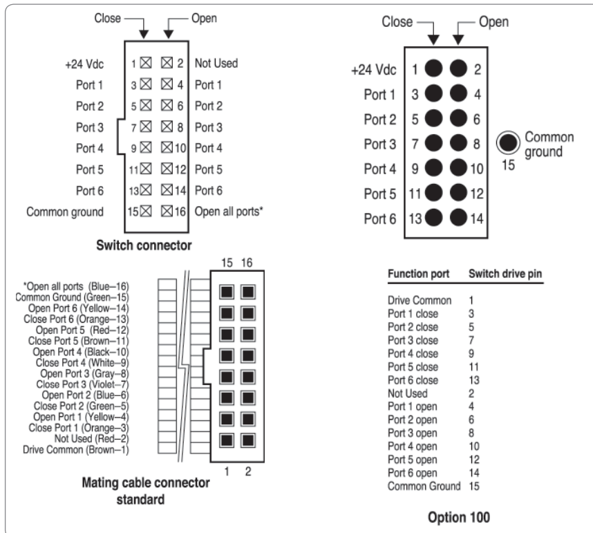
Figure 7. Drive connection diagrams
