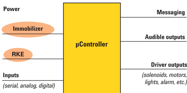
Figure 1: Body control module (with remote keyless entry & immobilizer)
