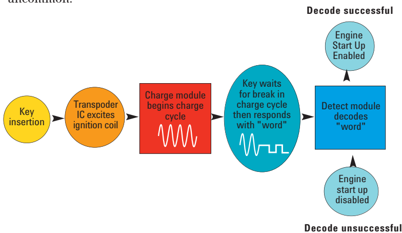
Figure 3: Immobilizer functionality action flow
