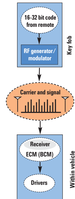
Figure 2: RKE functionality action flow
