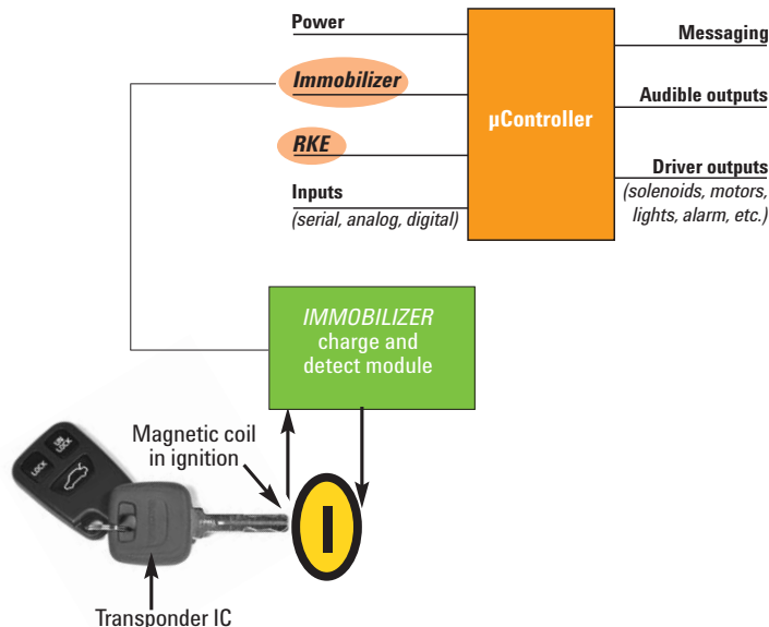
Figure 4: Immobilizer
