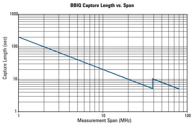
Figure 3b. MXA (BBIQ mode) capture length vs. span
