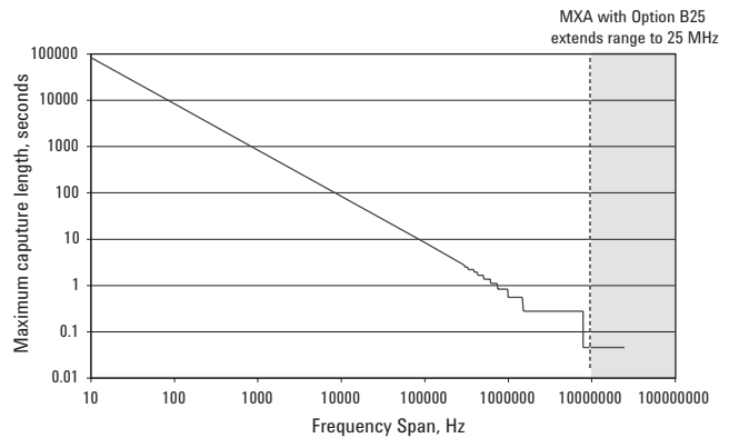
Figure 3a. MXA (RF mode) and EXA capture length
