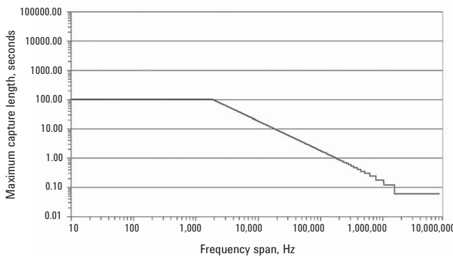
Figure 2. PSA capture length
