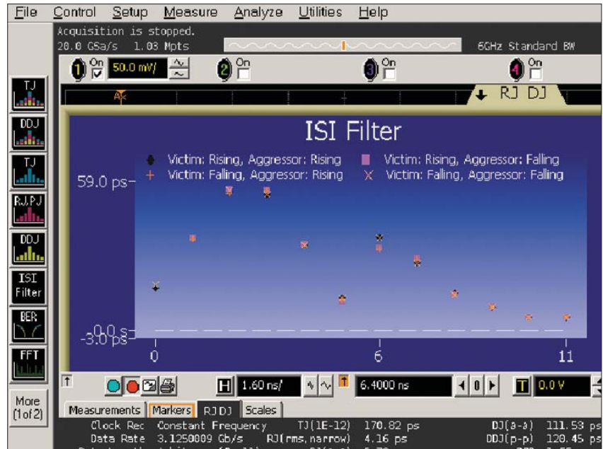
Figure 7. EZJIT Plus modeled the example signal’s DDJ with this ISI filter when the lead value was set to 0 and the lag value was set to 11.
