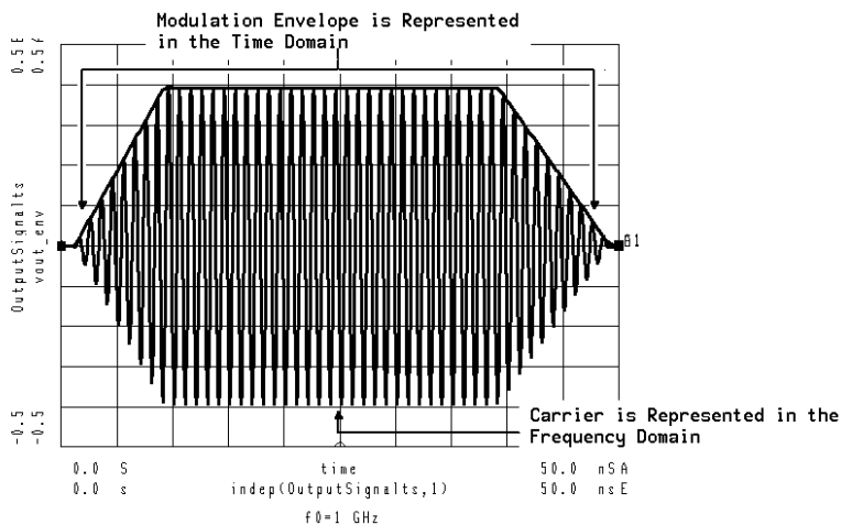
Figure 1-1. Modulated signal in the time domain
