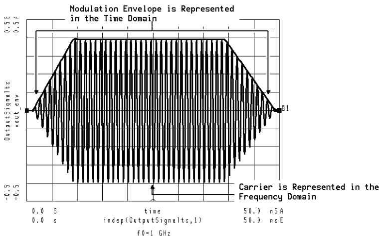
Figure 1-3. Modulated signal in the time domain
