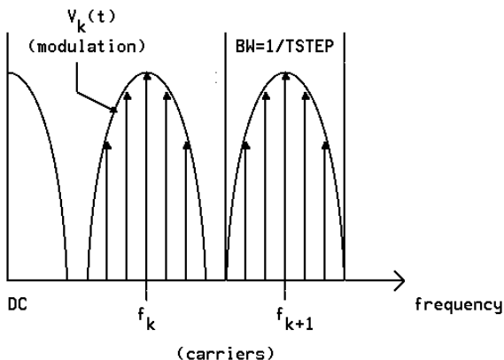
Figure 1-4. Spectra in the frequency domain
