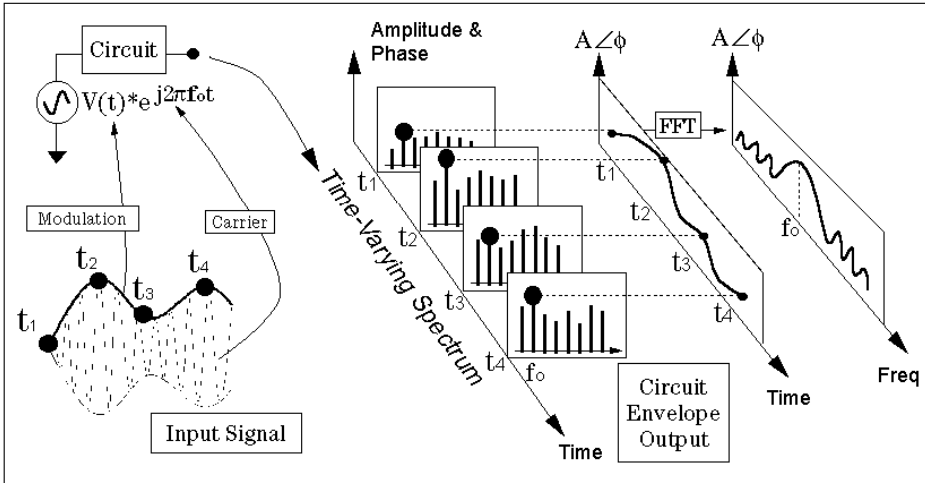
Figure 1-5. A Modulated signal and its simulated time-varying spectrum
