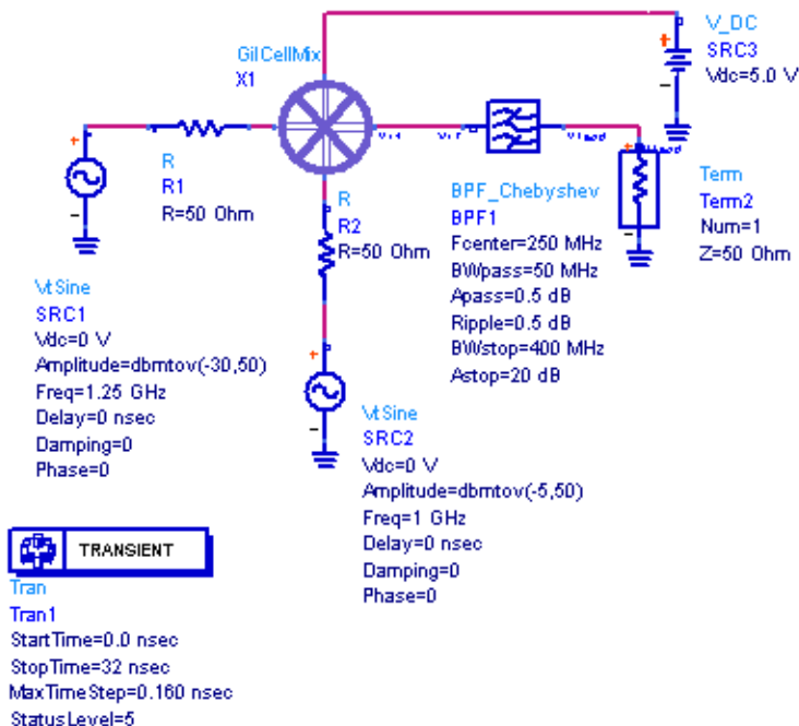
Figure 1-1. Setup for Transient/Convolution simulation
