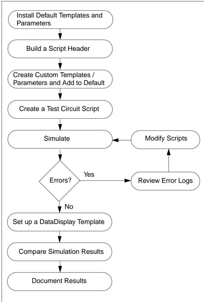
Figure 1-1. Design Kit Model Verification Process Flow
