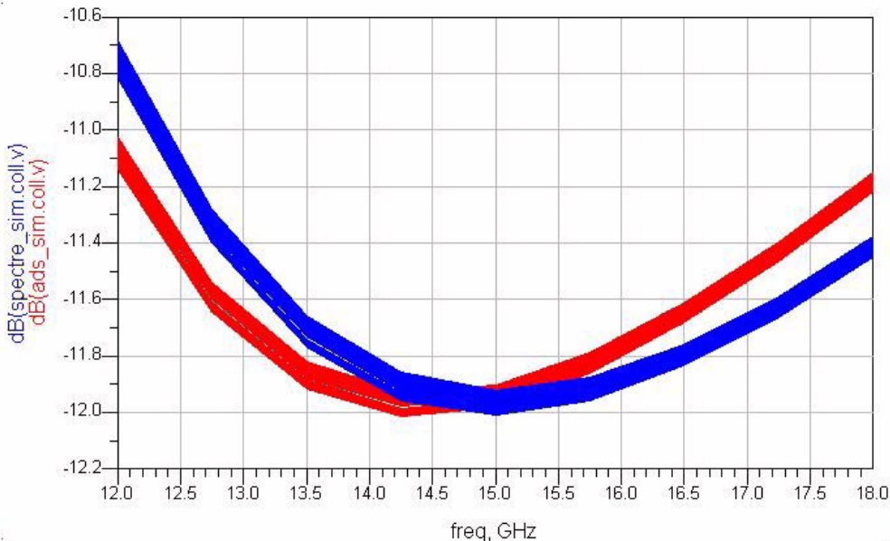
Figure 4-2. Monte Carlo Results
