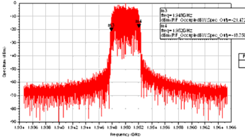
Meas Spectrum with Maximum Power
