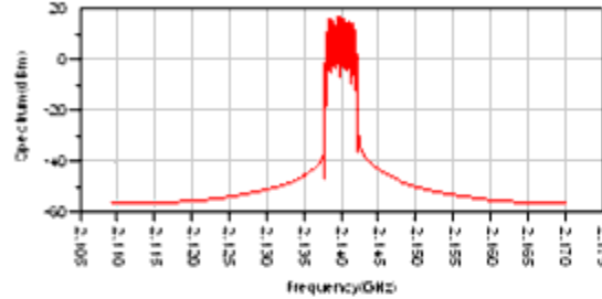
Spectrum of 10MHz and 5 MHz Higher than Main Channel
