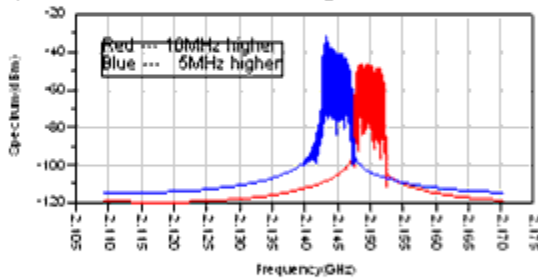
Spectrum of 10MHz and 5 MHz Higher than Main Channel
