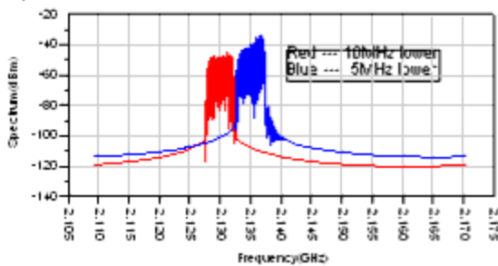
Spectrum of 10MHz and 5 MHz Lower than Main Channel
