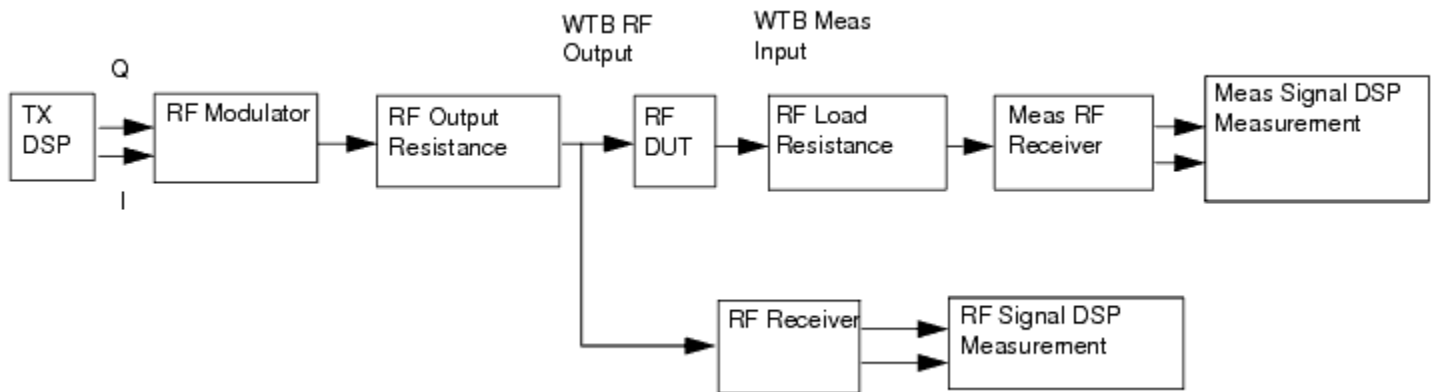
Transmitter Wireless Test Bench Block Diagram
