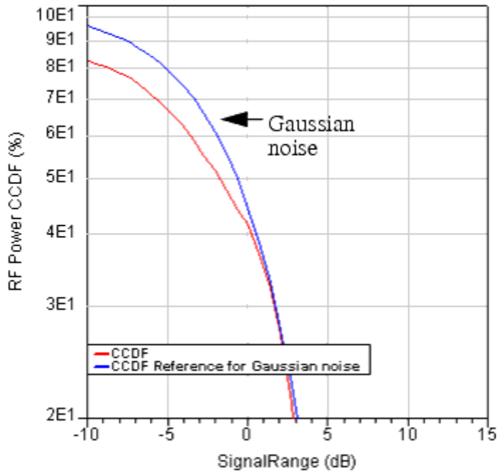
RF Power Complementary Cumulative Distribution Function (CCDF)
