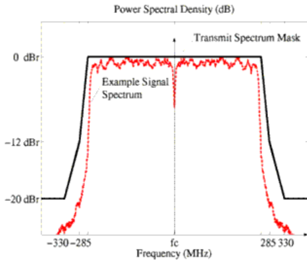
Transmit Spectrum Mask
