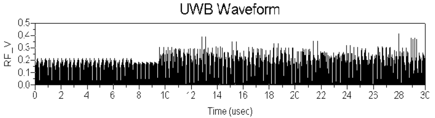
Time Envelope of UWB RF Signal for Default Settings (one frame)
