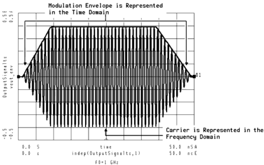
Modulated signal in the time domain
