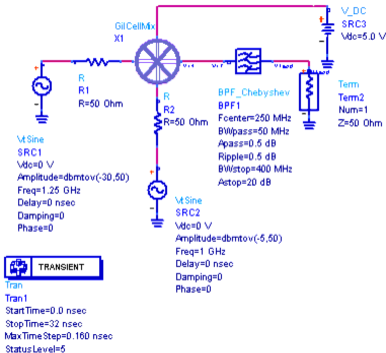
Setup for Transient/Convolution simulation
