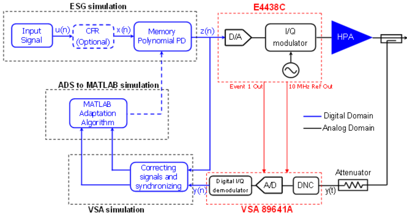
The block diagram of the digital predistortion with memory effects and CFR
