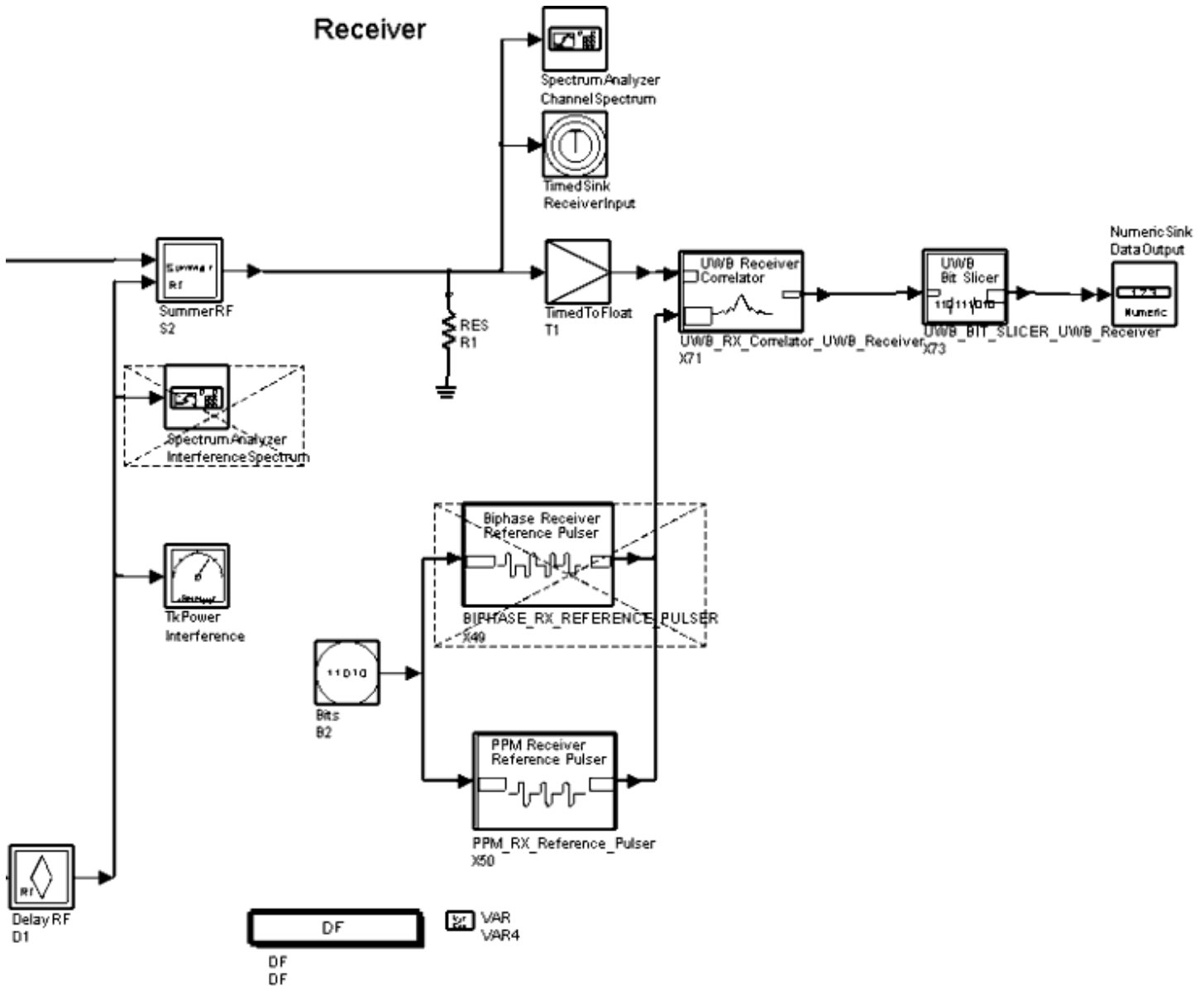
Wide Band Interference Test Bench, Receiver
