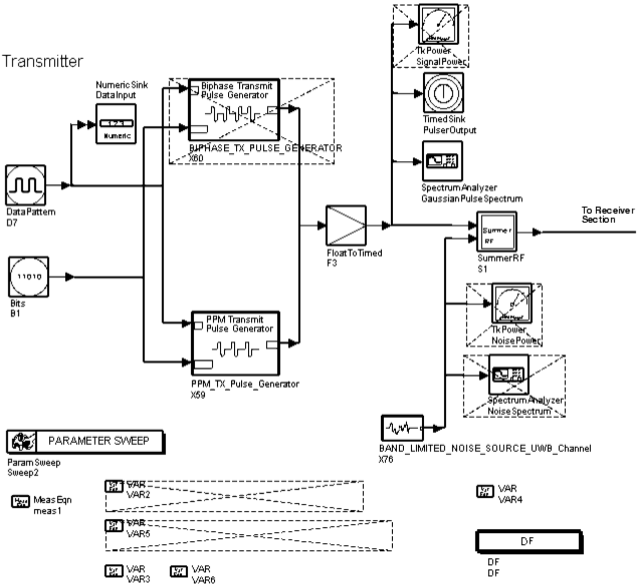
Pulse Position Modulation Test Bench, Transmitter Section
