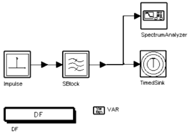
HighPassFilter_RFSim.dsn Schematic
