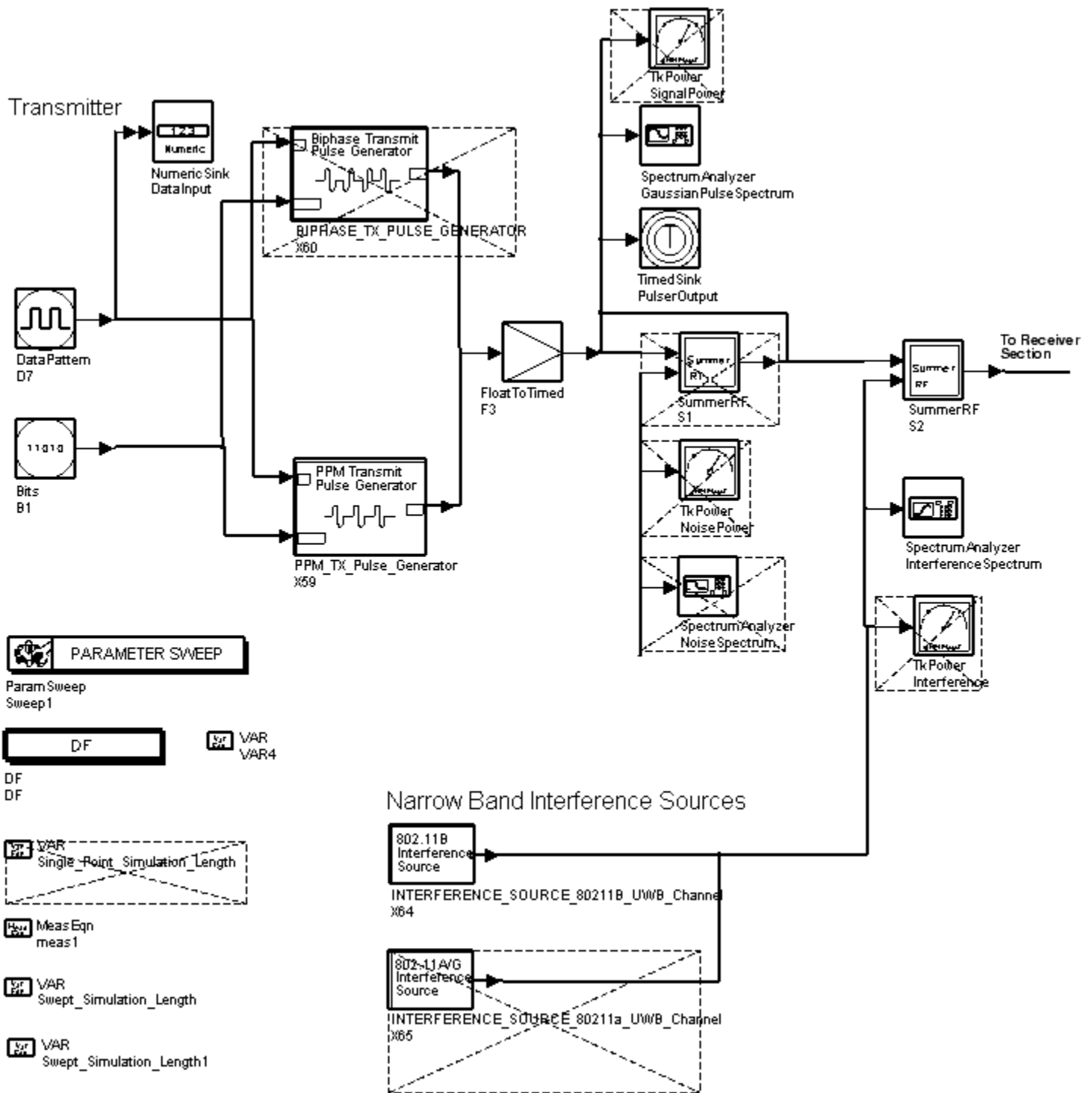
Narrow Band Test Bench, Transmitter Section
