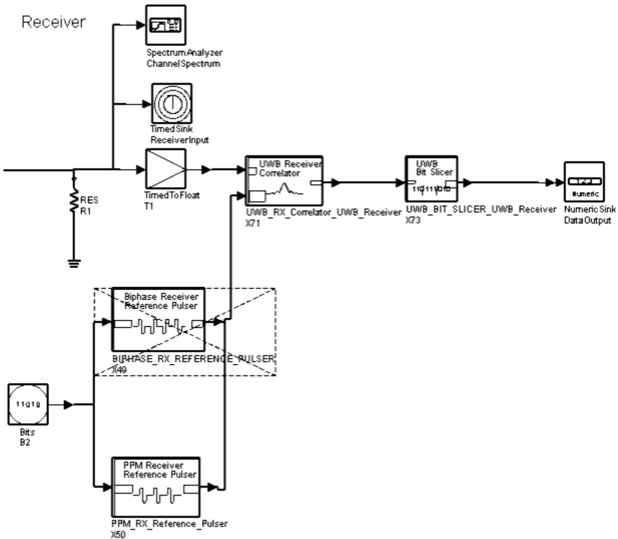
Narrow Band Test Bench, Receiver Section
