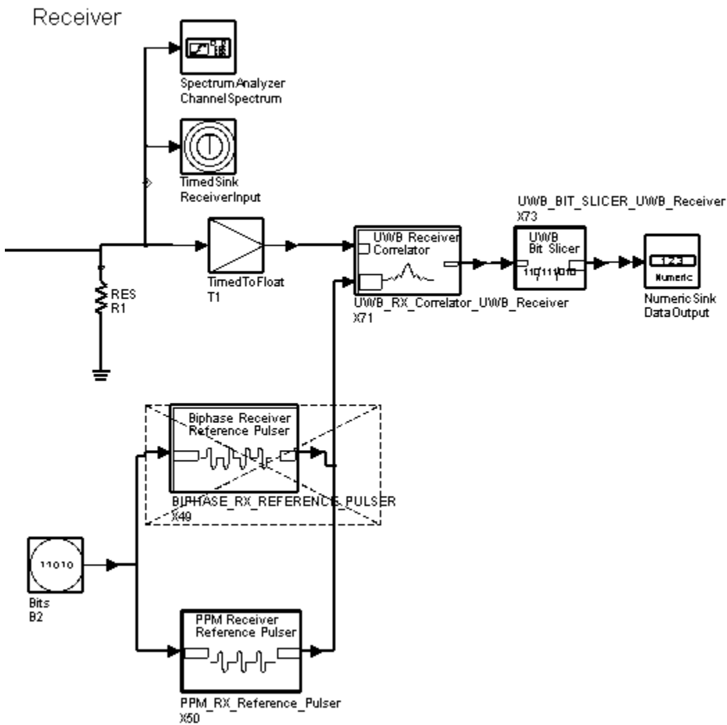
Pulse Position Modulation Test Bench, Receiver Section
