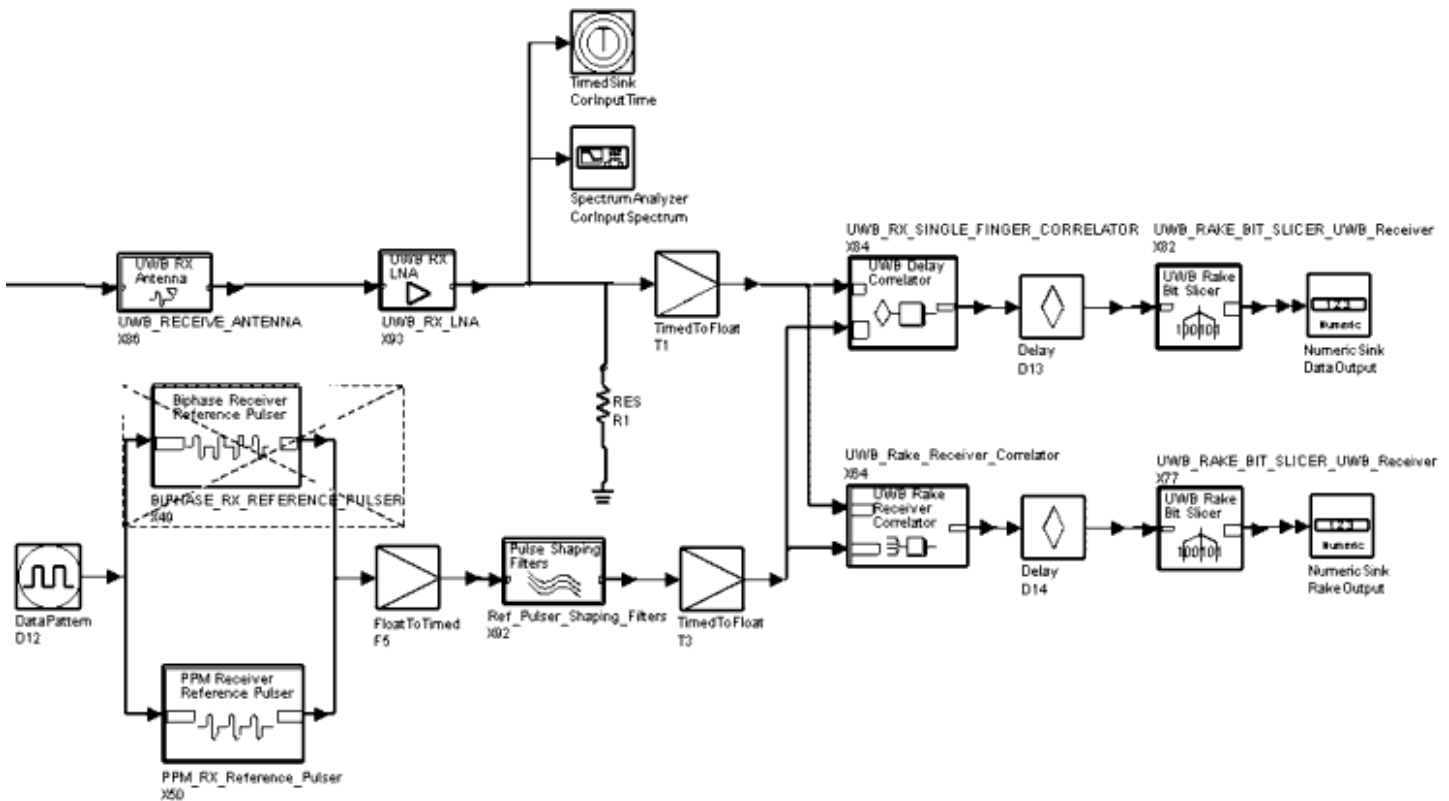
Rake Receiver Test Bench Schematic, Receiver Section
