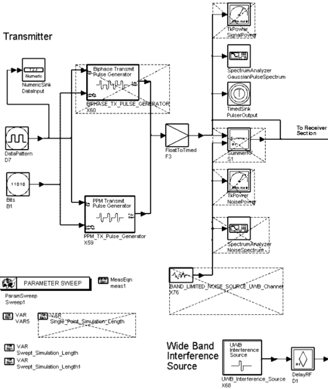
Wide Band Interference Test Bench, Transmitter Section
