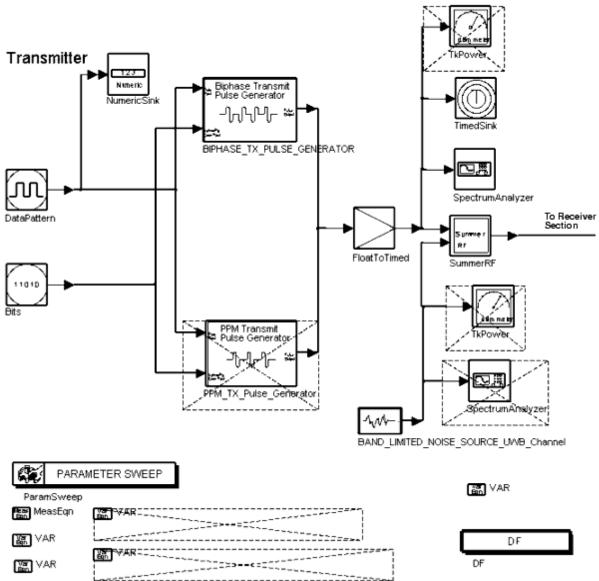
Bi-Phase Modulation Test Bench, Transmitter Section
