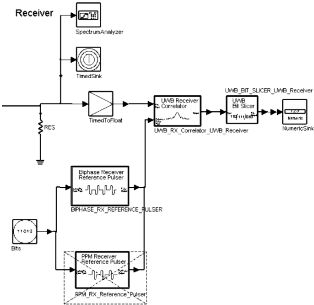
Bi-Phase Modulation Test Bench, Receiver Section
