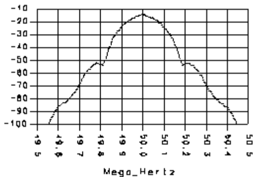
Power Spectrum of 0.3GMSK Modulator as Estimated by FFTAnalyzer Measurement
