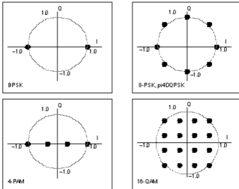
Examples of IQ-Constellations as Used in EVM Measurement
