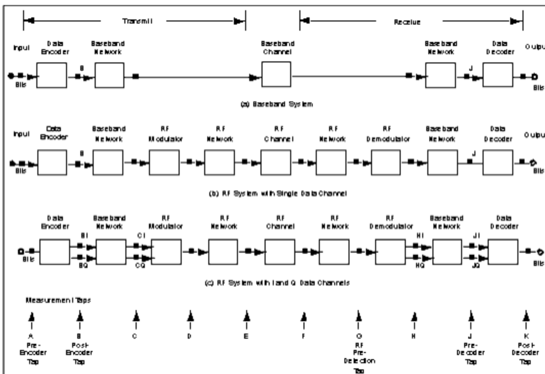
Typical Baseband and RF Systems
