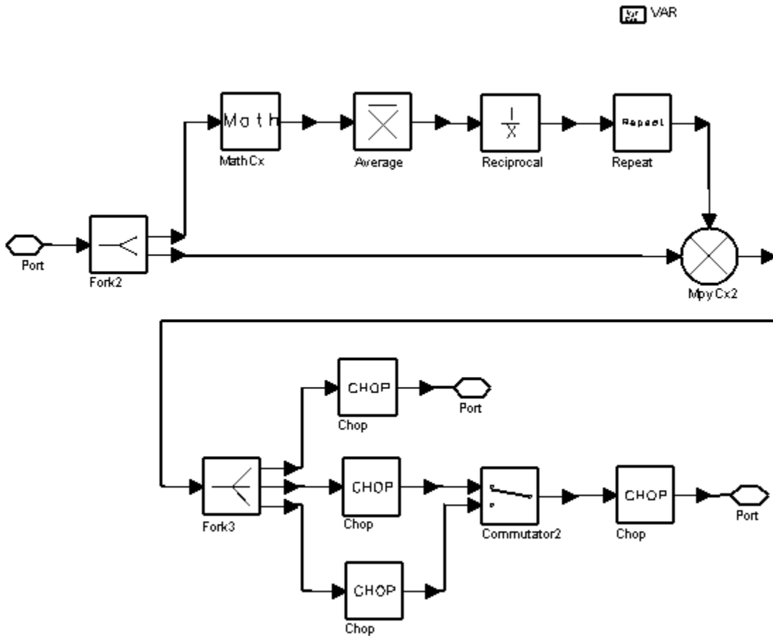
TDSCDMA_BurstDeMux Schematic
