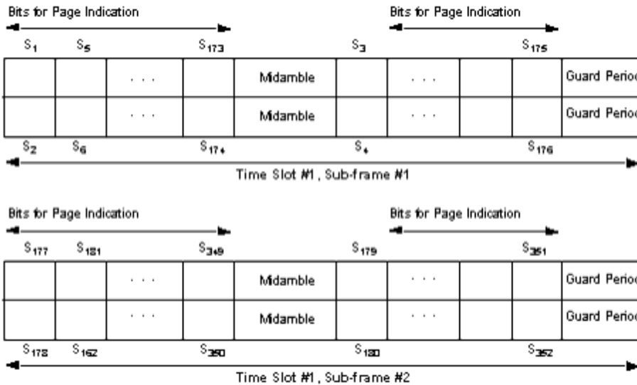
Transmission of Paging Indicator Carrying Bits in PICH Bursts
