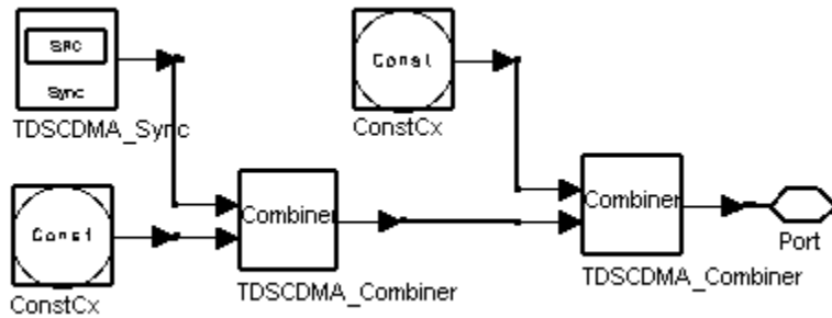
TDSCDMA_DwPCH Schematic
