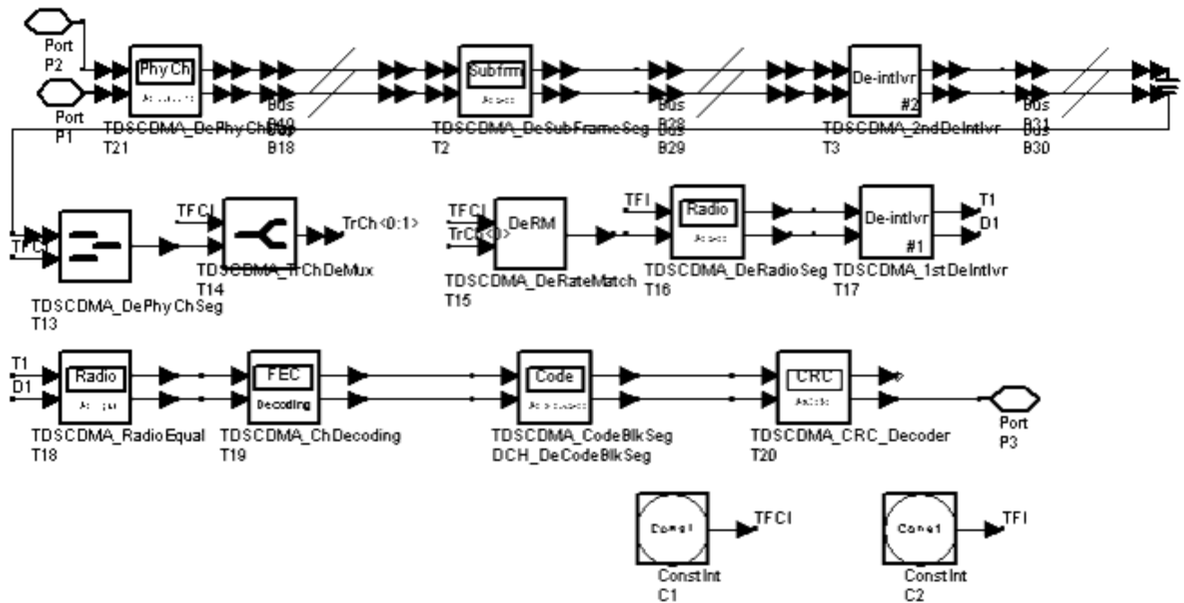
TDSCDMA_RefChDecoder Schematic
