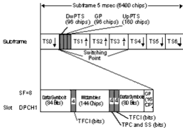
Subframe Structure of 12.2 kbps Uplink Channel
