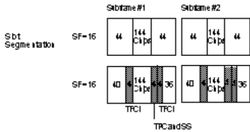
Frame Structure of 12.2 kbps Downlink Channel
