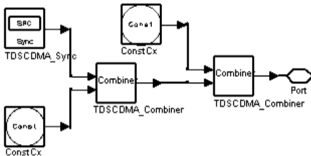
TDSCDMA_UpPCH Schematic
