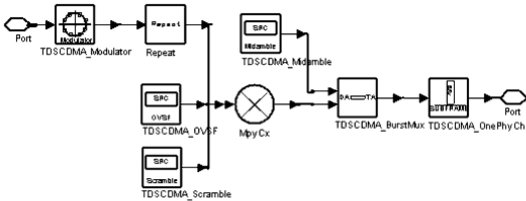
TDSCDMA_FPACH Schematic
