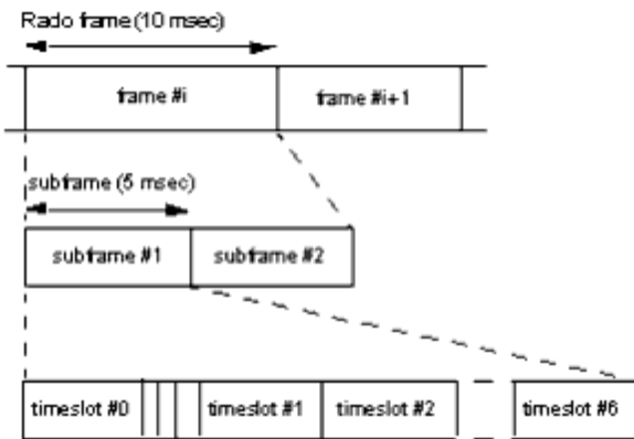
Physical Channel Signal Format
