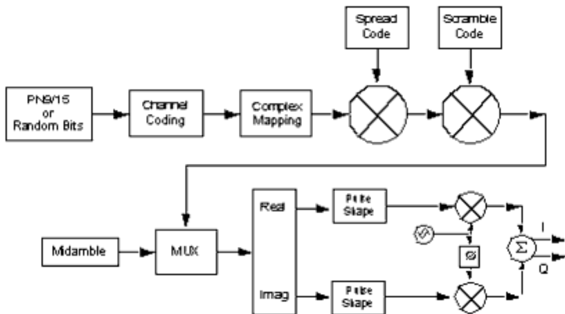
Physical Channel Transmitter Structure
