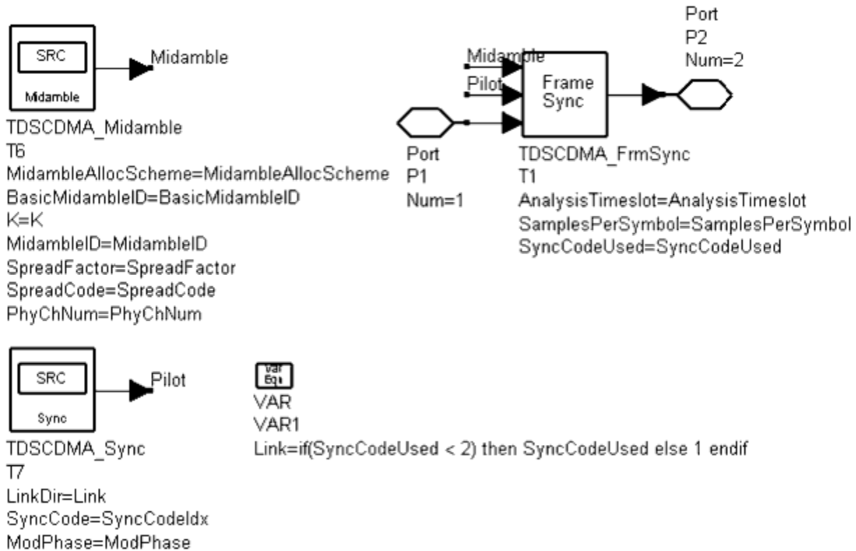
TDSCDMA_FrameSync Schematic
