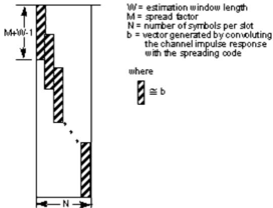
Structure of Matrix A
