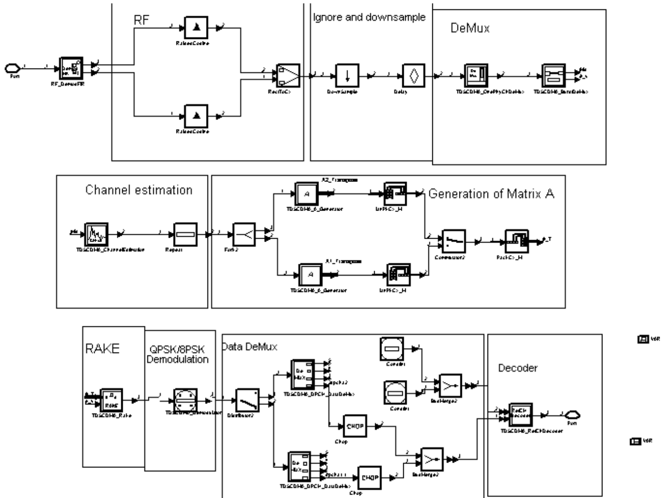
TDSCDMA_12_2_DL_RakeReceiver Schematic
