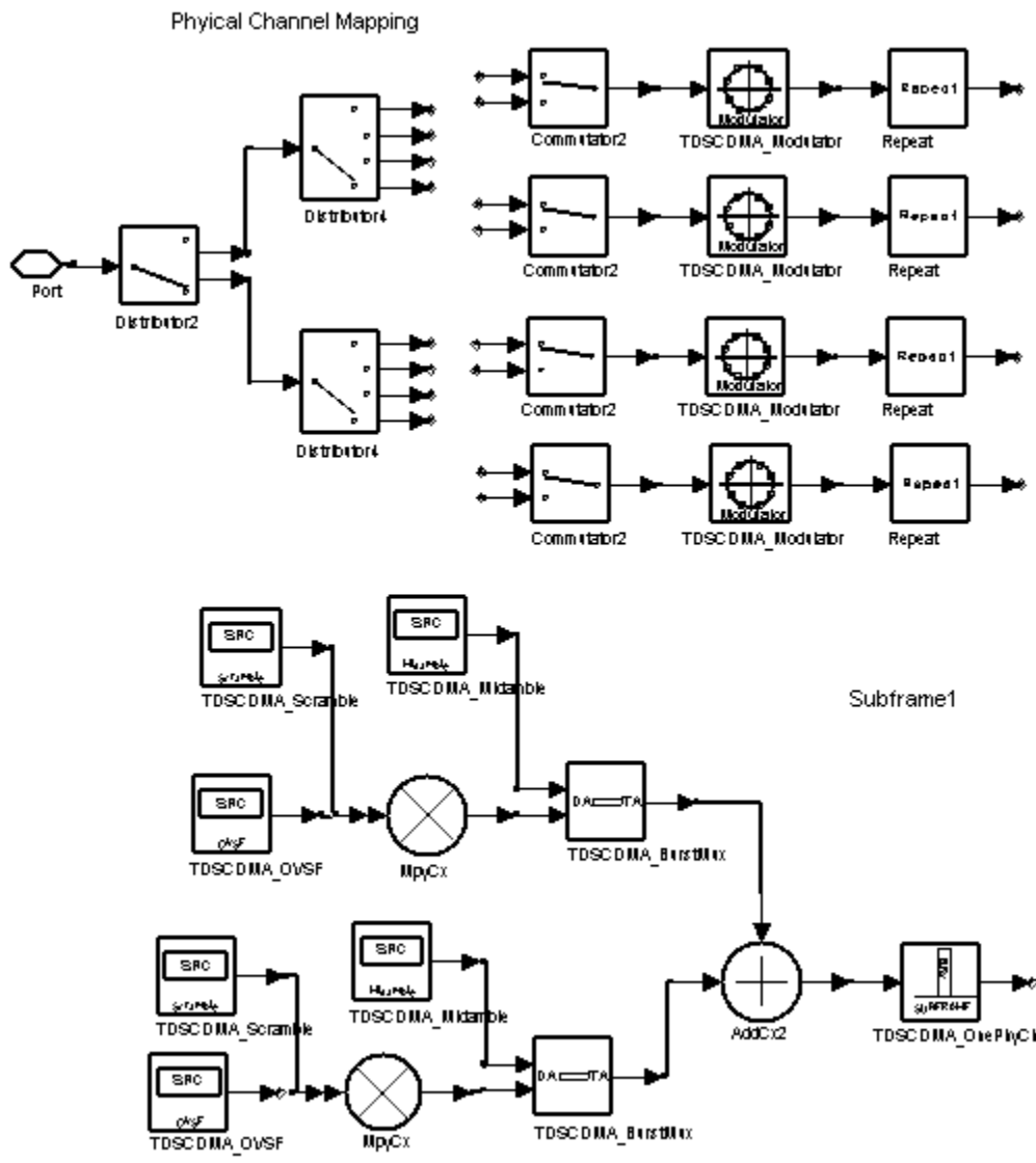
TDSCDMA_PICH Schematic (1 of 2)
