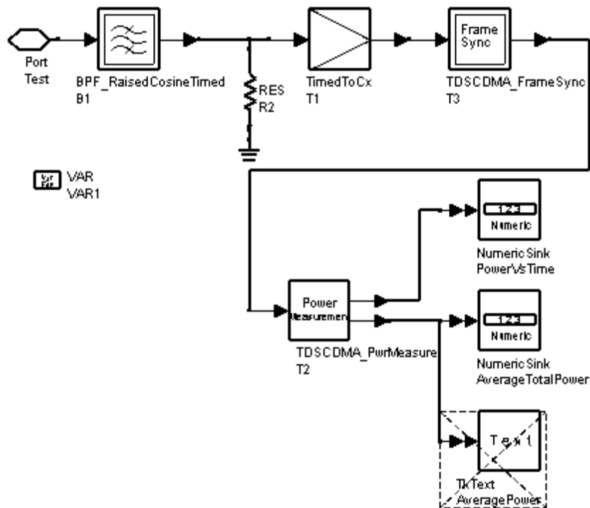
TDSCDMA_RF_PwrMeasure Schematic
