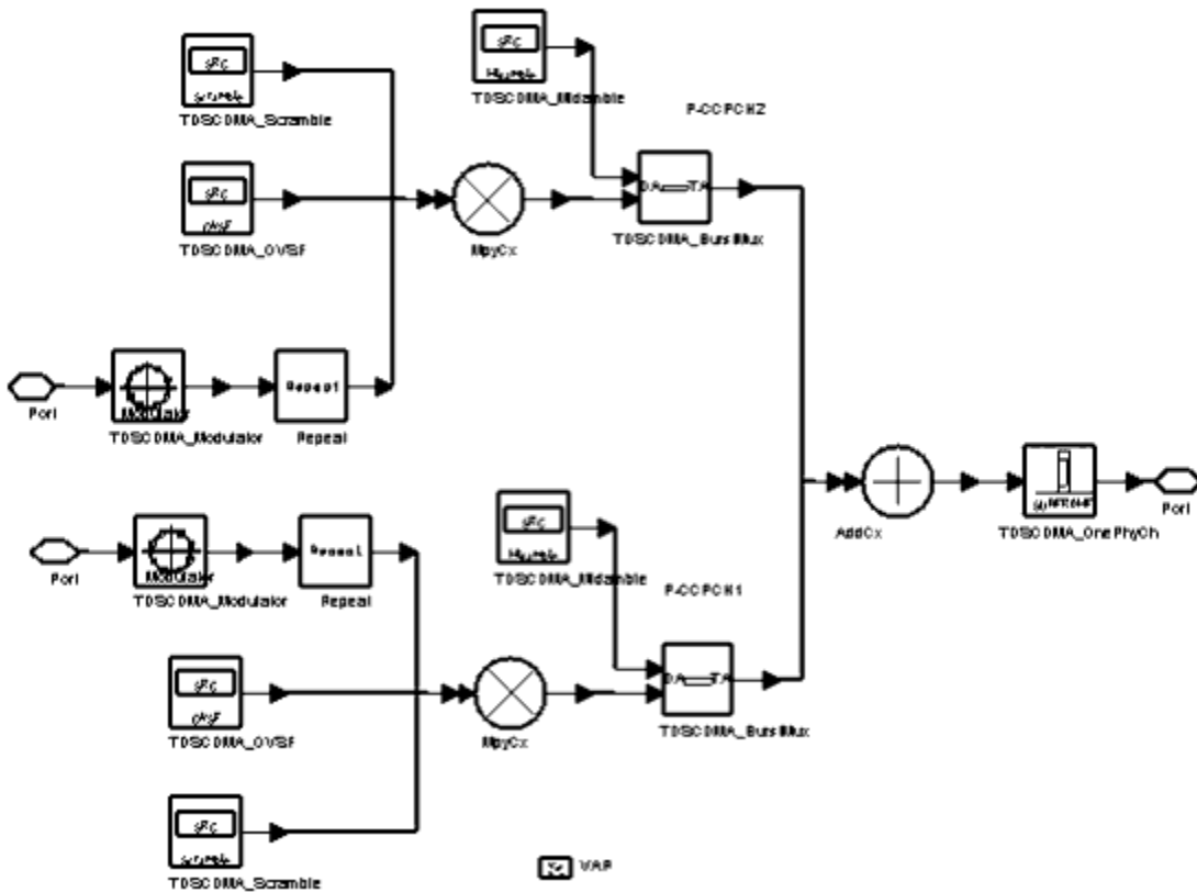
TDSCDMA_PCCPCH Schematic
