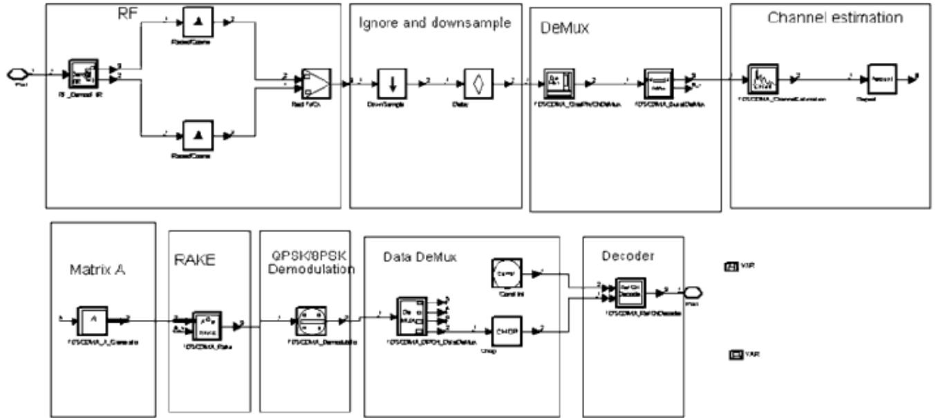
TDSCDMA_12_2_UL_RakeReceiver Schematic
