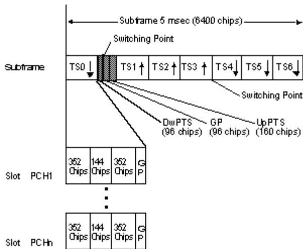
Example of a SubFrame Structure
