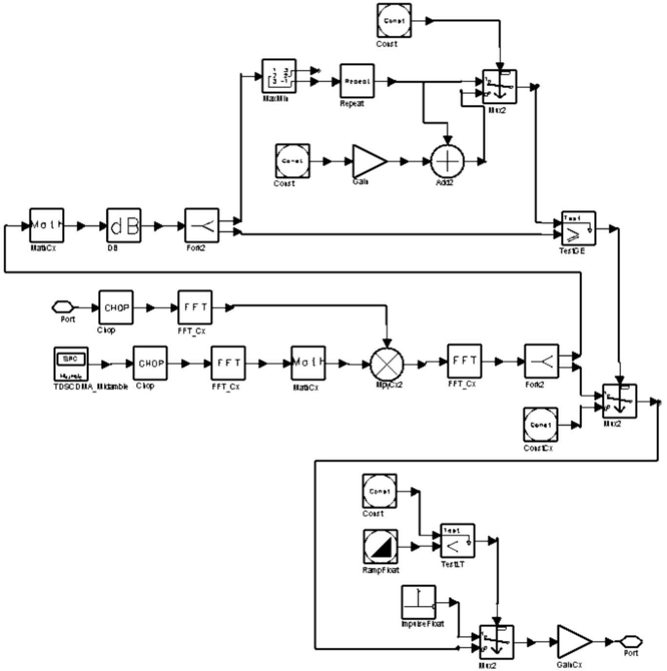
TDSCDMA_ChannelEstimation Schematic
