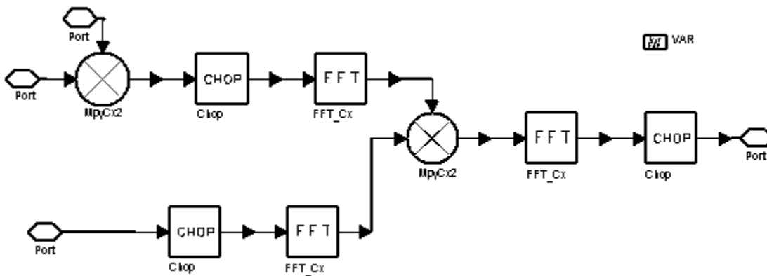
TDSCDMA_b_k_Generator Schematic
