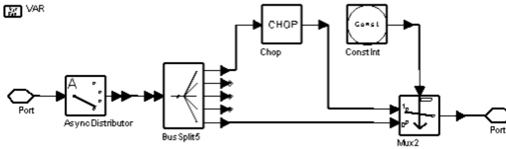
TDSCDMA_OnePhyChDeMux Schematic
