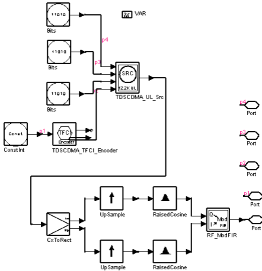
TDSCDMA_UL_RF Schematic
