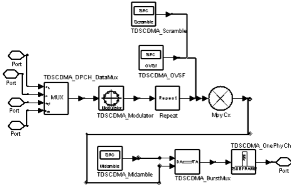
TDSCDMA_DPCH Schematic
