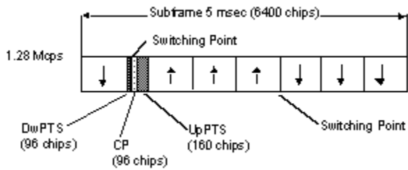
Structure of Subframe for 1.28Mcps TDD Option
