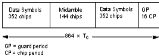
Burst Structure of Traffic Burst Format
