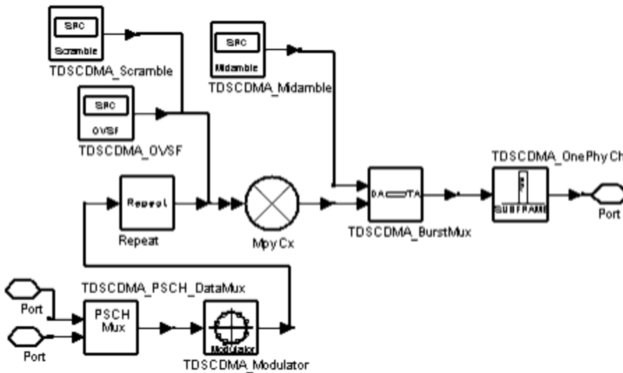
TDSCDMA_PSCH Schematic
