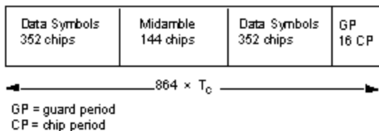
Burst Structure of Traffic Burst Format
