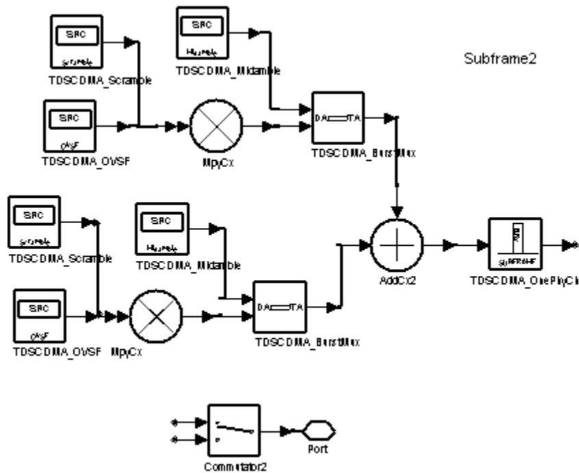
TDSCDMA_PICH Schematic (2 of 2)
