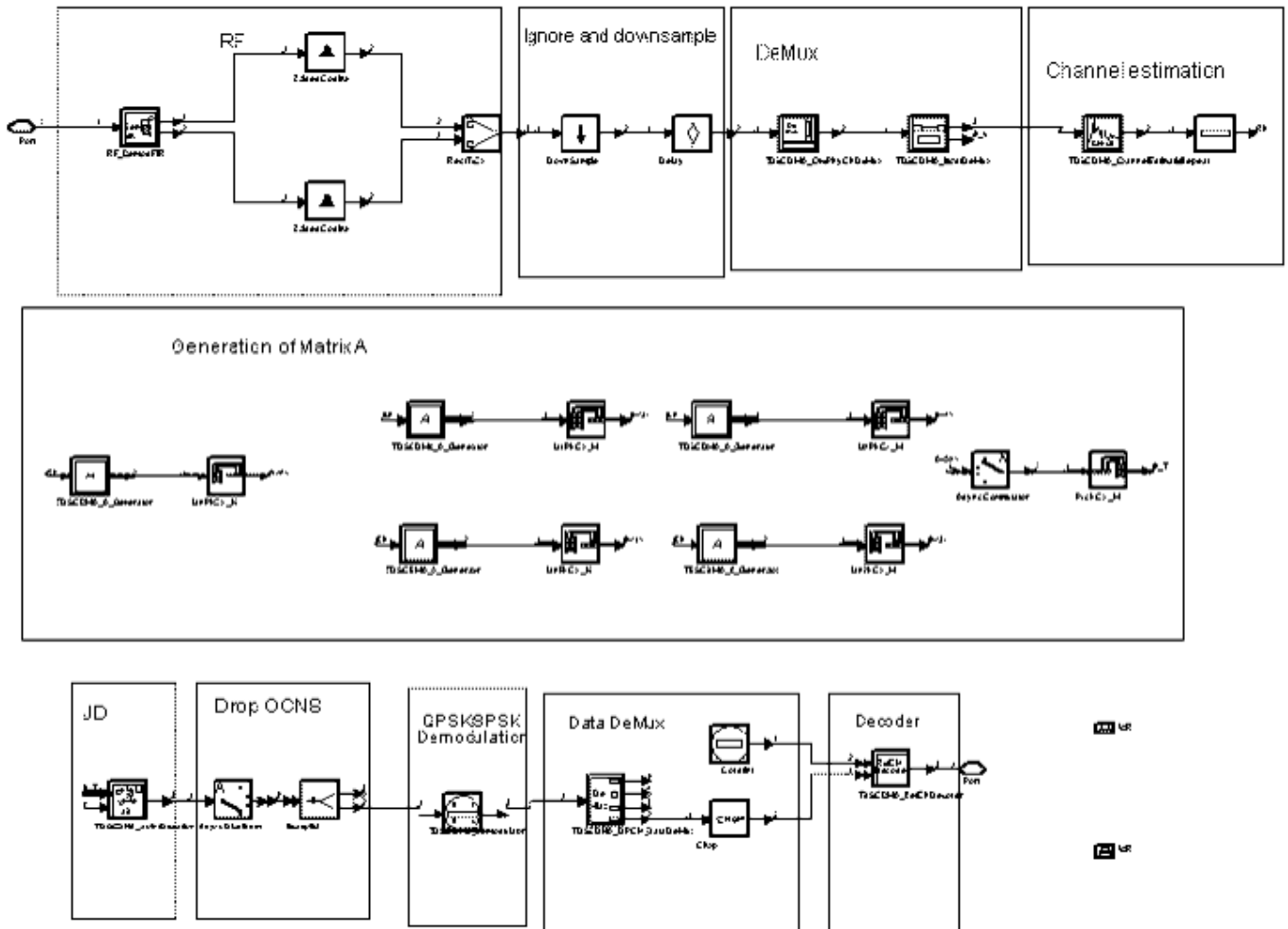
TDSCDMA_12_2_UL_JD_Receiver Schematic
