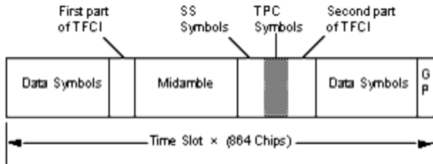
TDSCDMA Slot Structure
