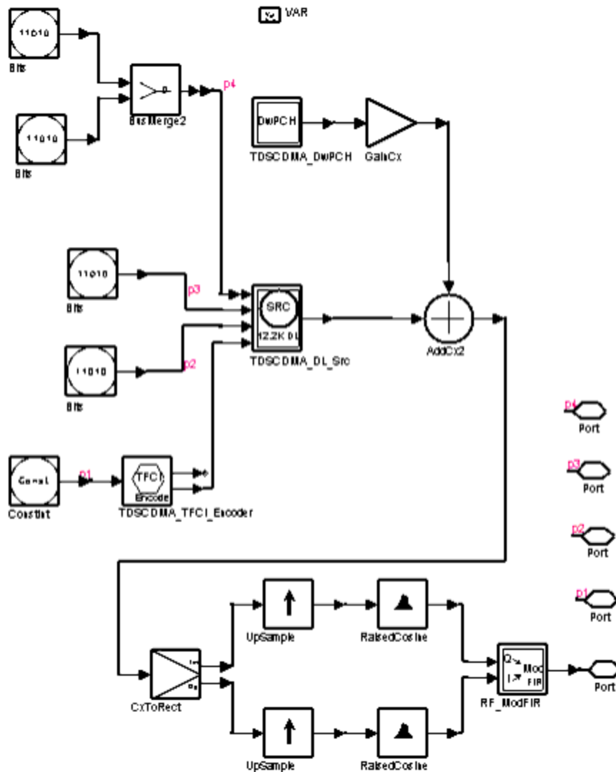
TDSCDMA_DL_RF Schematic
