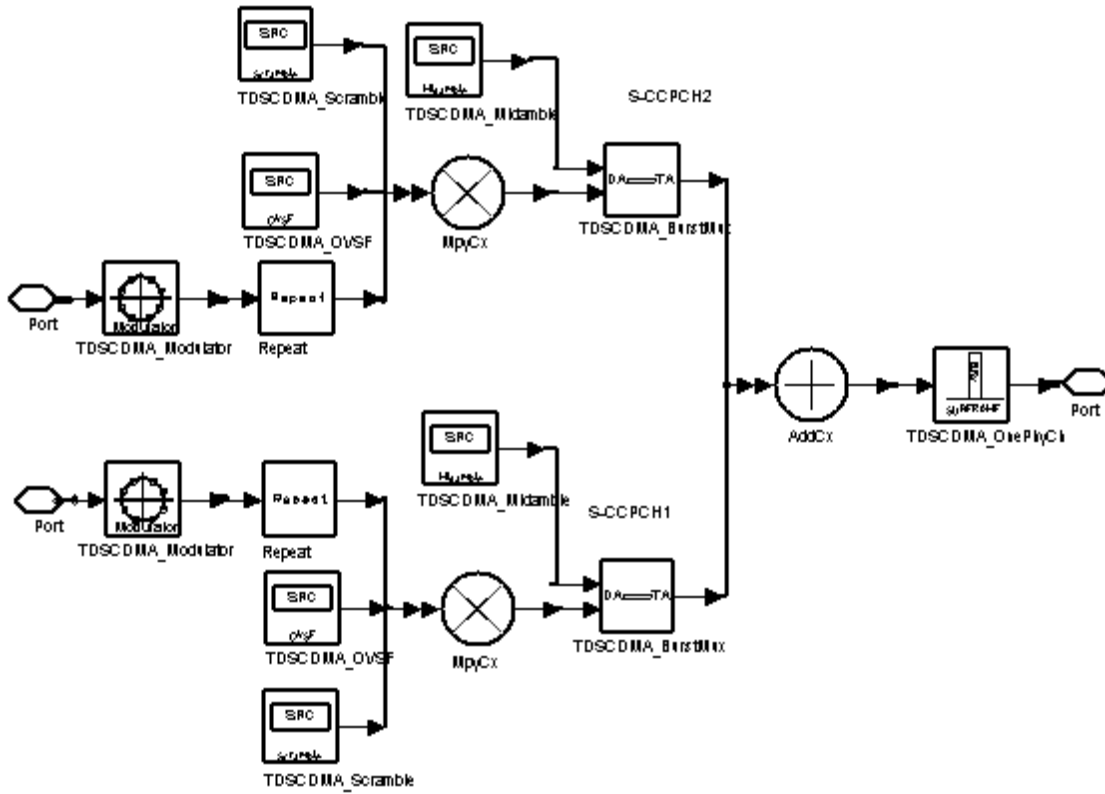
TDSCDMA_SCCPCH Schematic
