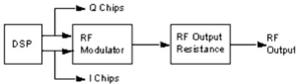
Signal Source Block Diagram
