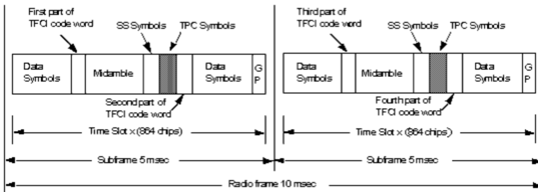
Burst Structure
