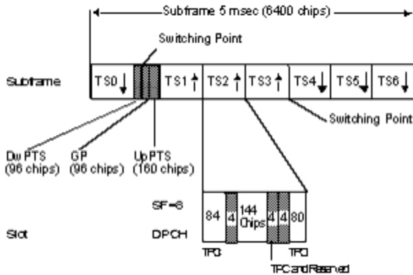
SubFrame Structure of 12.2 kbps Uplink Channel
