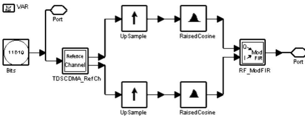
TDSCDMA_RefCh_RF Schematic
