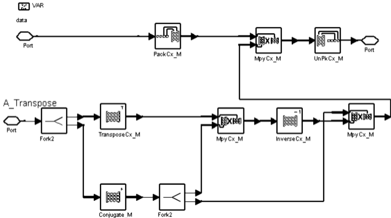
TDSCDMA_JointDetection Schematic
