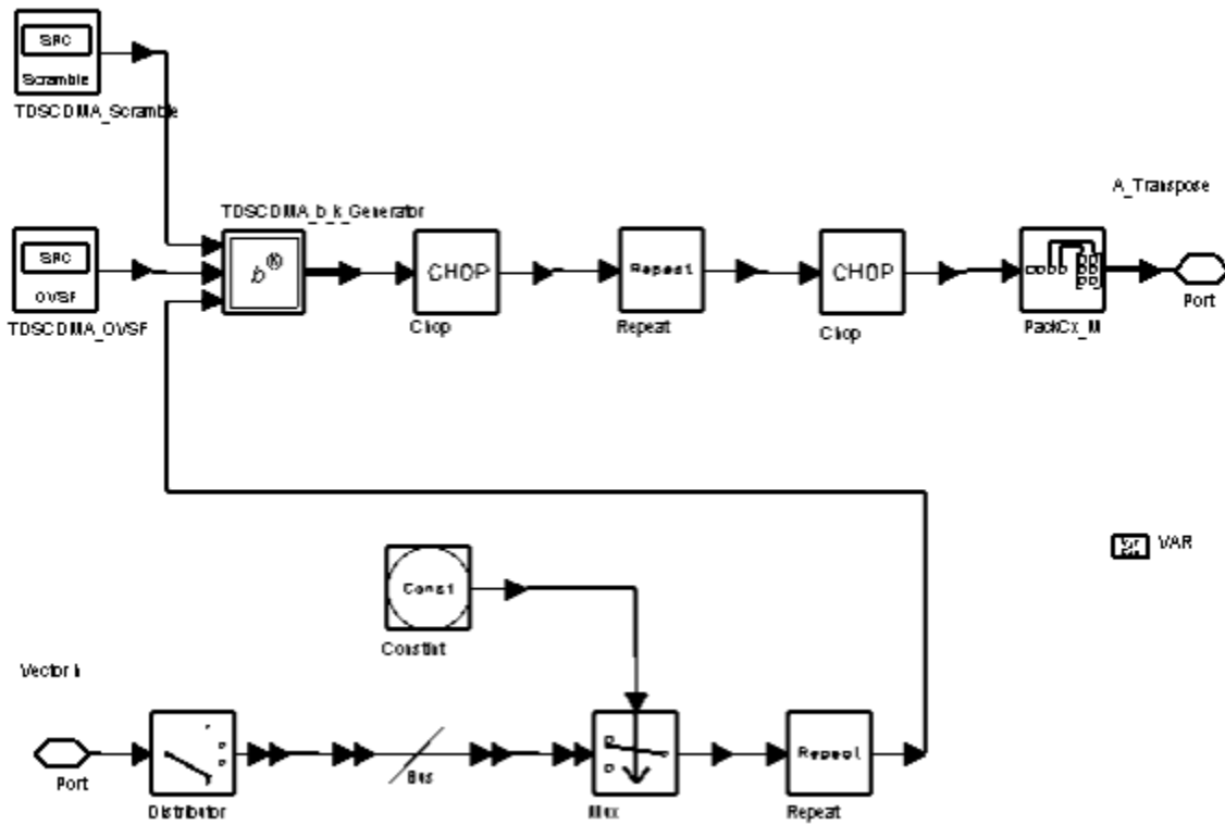
TDSCDMA_A_Generator Schematic
