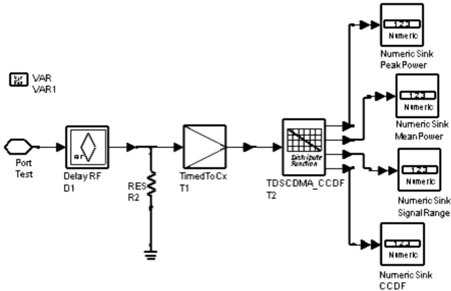
TDSCDMA_RF_CCDF Schematic
