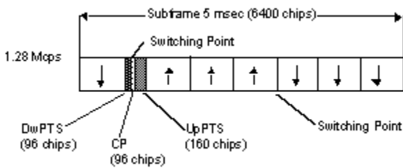
Sub-Frame Structure for 1.28Mcps TDD Option
