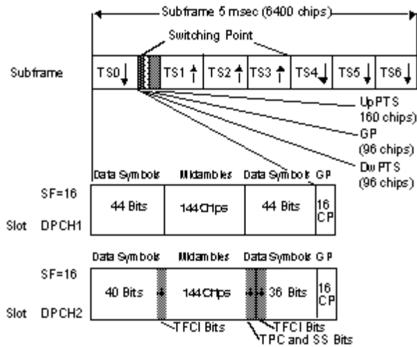
Subframe Structure of 12.2 kbps DL Channel
