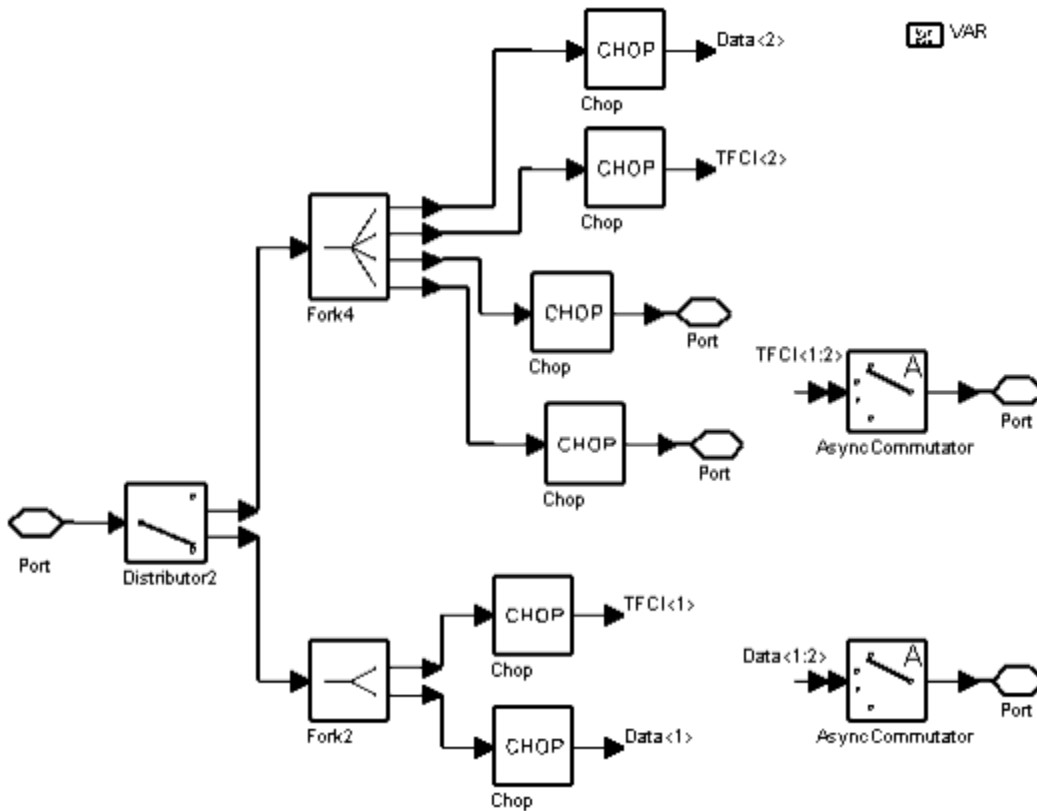
TDSCDMA_DPCH_DataDeMux Schematic
