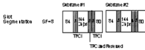
Frame Structure of 12.2 kbps UL Channel
