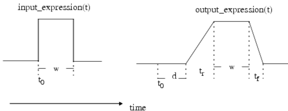
Transition Filter on Pulse Waveform
