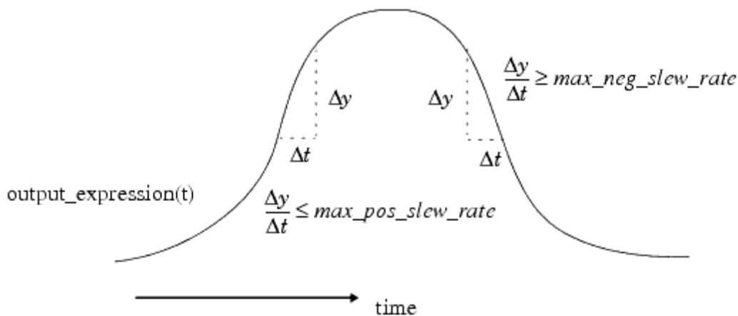
Slew Rate Limiting of Slope
